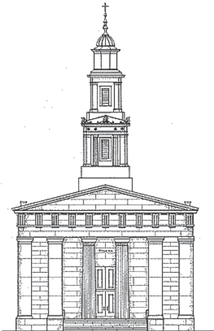
Christ Church Front Elevation
