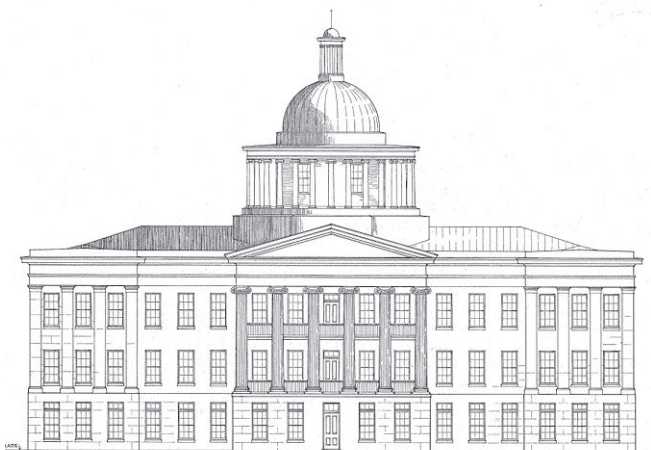
Barton Academy Front Elevation
